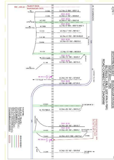
WESTERN RAILWAY BHAYANGAR DIVISION SEPTUARY-PBR BETWEEN: ISIR, PBR, KLS PBR ROAD CONNECTIVITY DIAGRAM
